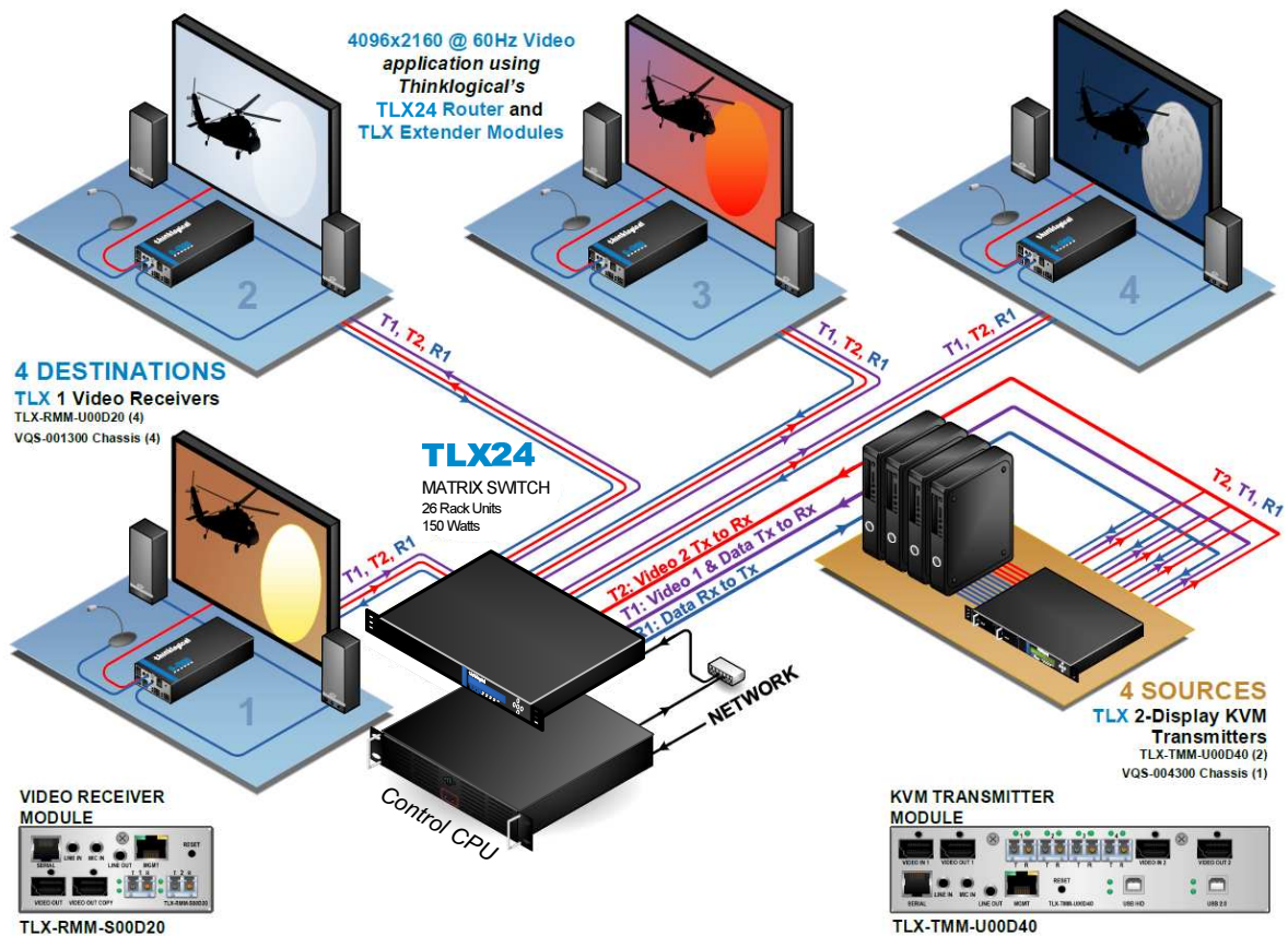
Figure 2b. Typical TOE TLX24 Matrix Switch (w/o Front Control Panel)
