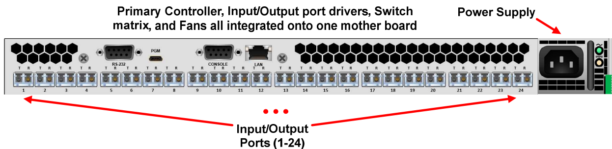
Figure 1a. Thinklogical TLX24 Matrix Switch
