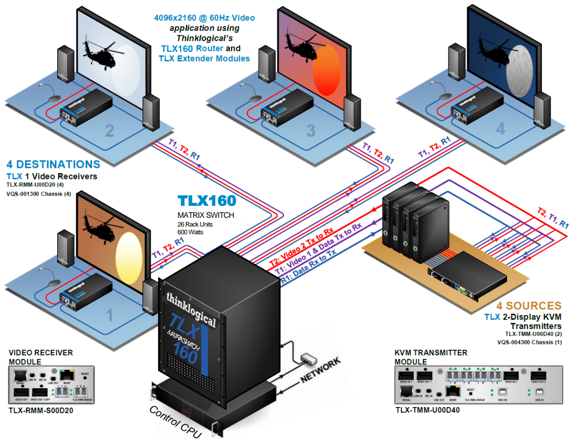
Figure 2a. Typical TOE TLX160 Matrix Switch
