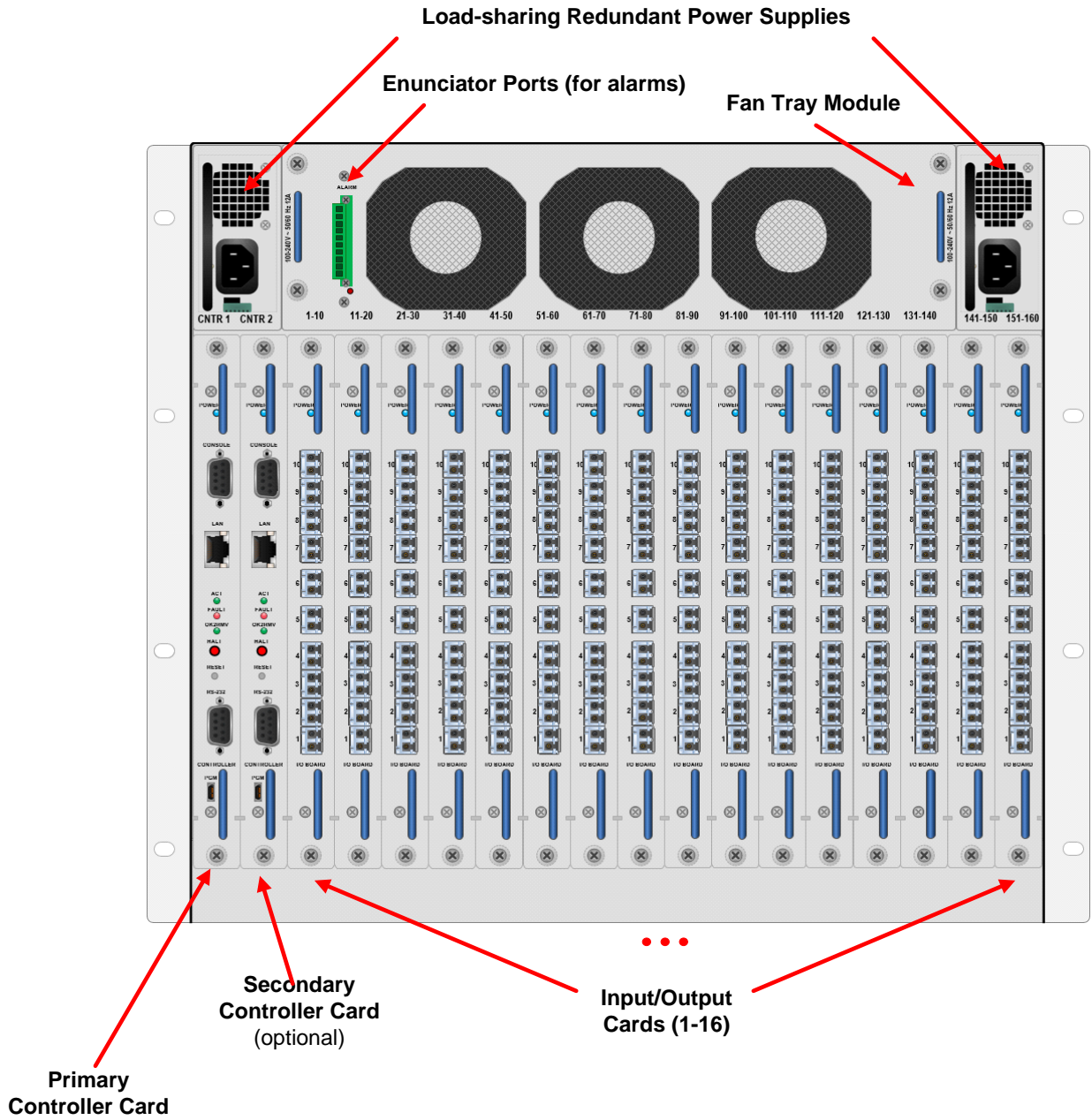
Figure 1a. Thinklogical TLX160 Matrix Switch
