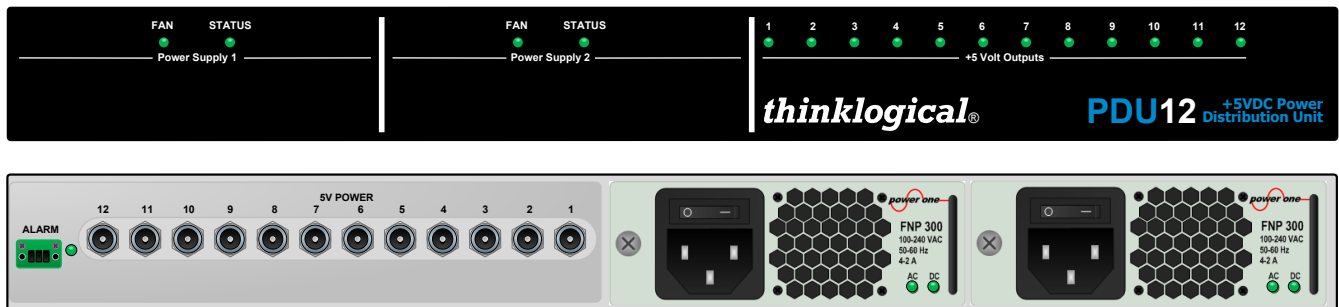
PDU12 Chassis, Part No. PDU-000012
