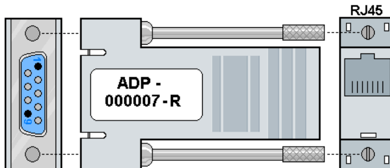
RJ45F to DB9M adapter for SCS/CFL
