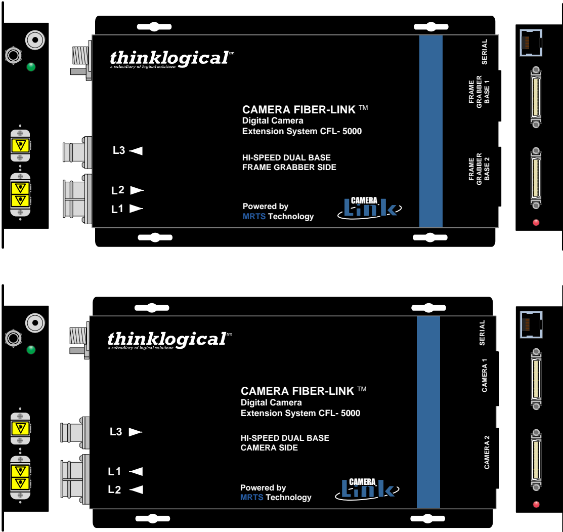
Figure 4: Top and side views of CFL-5000 Camera Side and Frame Grabber Side.
