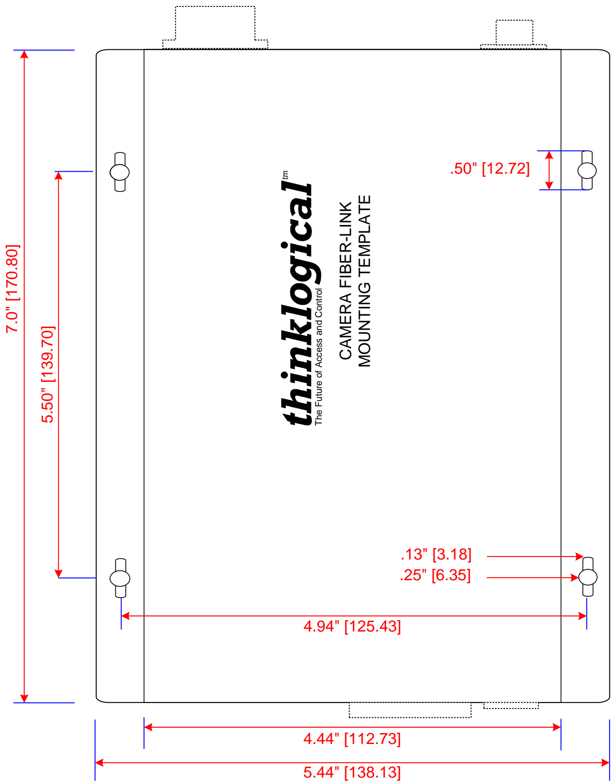
Figure 13: CFL Mounting Template
