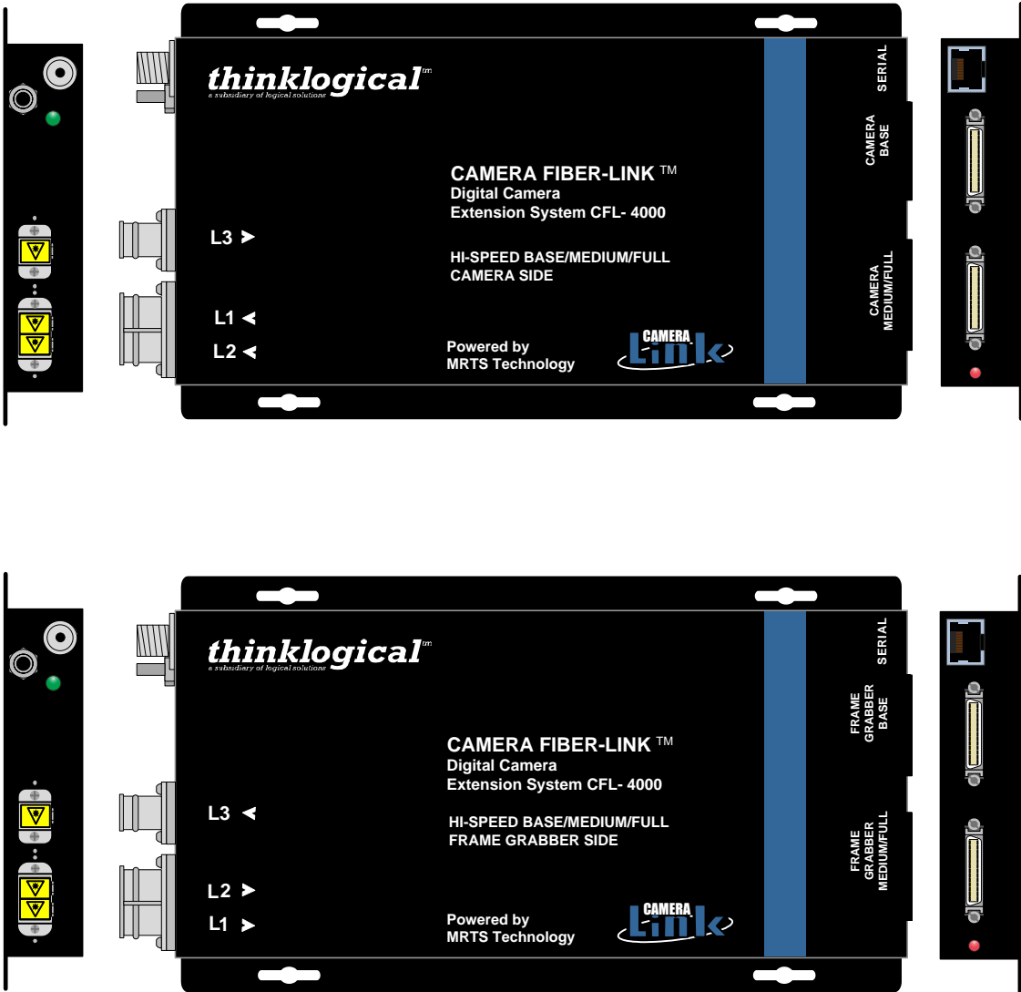
Figure 3: Top and side views of CFL-4000 Camera Side and Frame Grabber Side
