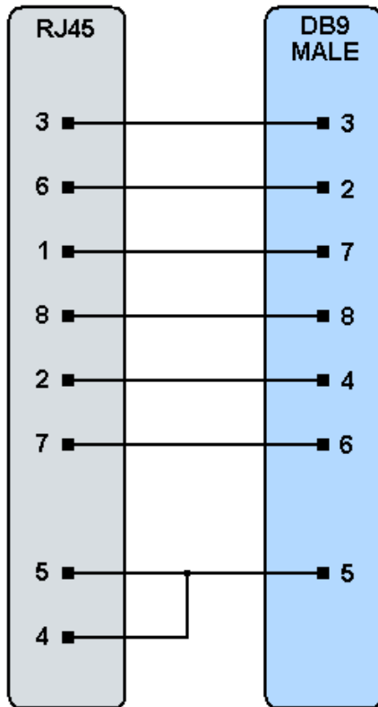
RJ45F to DB9M adapter for SCS/CFL
