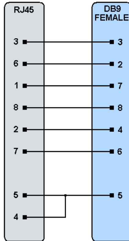
RJ45F to DB9F adapter for SCS/CFL
