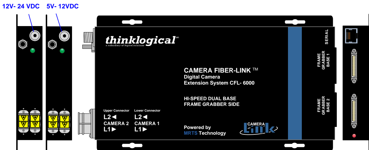
Figure 5: Top and side views of CFL-6000 Frame Grabber Side. The far left view shows the industrial enhancements (12V-24V Power) available.
